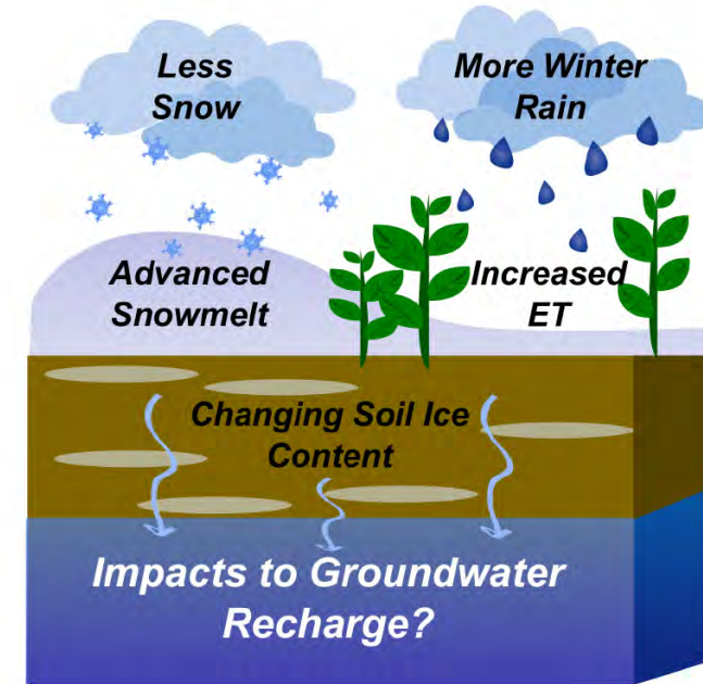
Figure 7: Conceptual diagram of climate change impacts to groundwater recharge.
